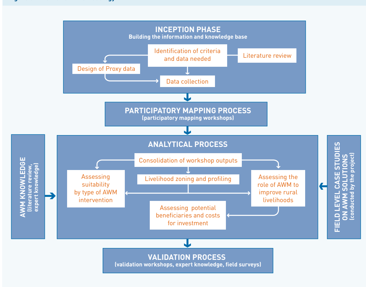
Figure 3 Framework methodology
